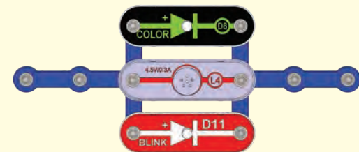
Parallel Circuit
